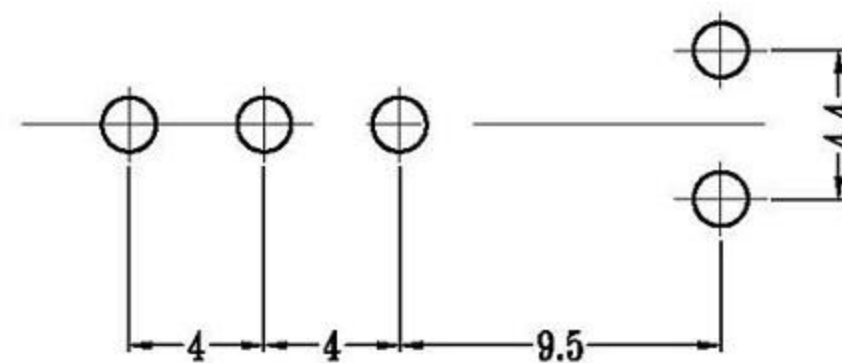
P.C.B LAYOUT BOTTOM VIEW
